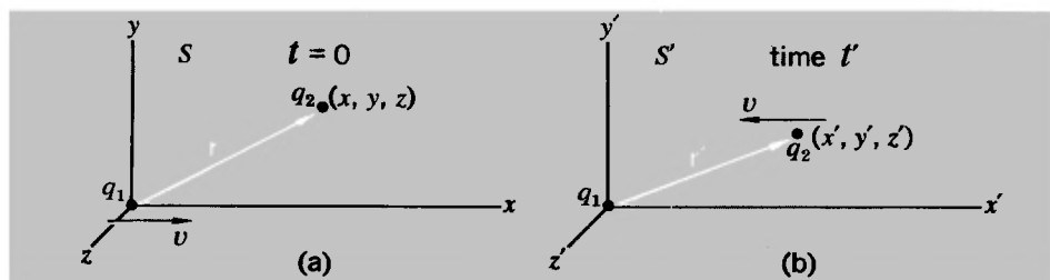
Fig. 8-4 (a) Moving source charge and stationary test charge in arbitrary relative positions. (b) The same situation transformed to a frame in which the source charge is stationary.
